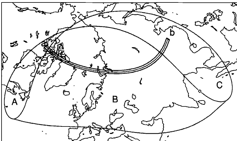
Total solformørkelse 1. august 2008
