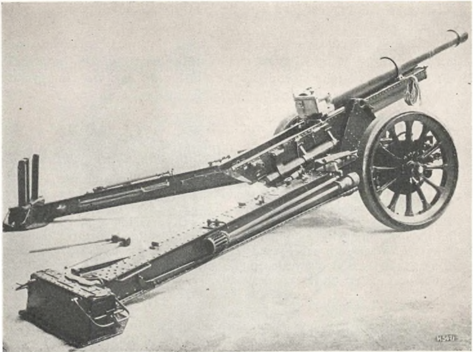
15 cm Felthaubits, Model 1929.
